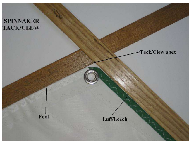
Photo 8 - Spinnaker Clew
