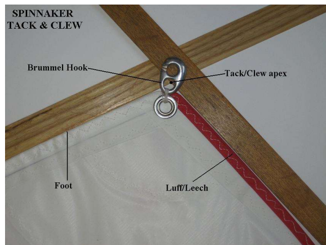
Photo 9 - Spinnaker Clew
