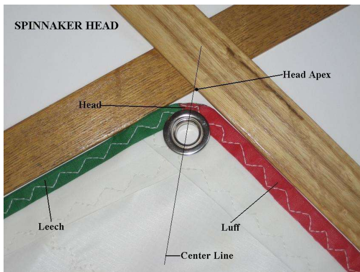
Photo 7 – Spinnaker Head
